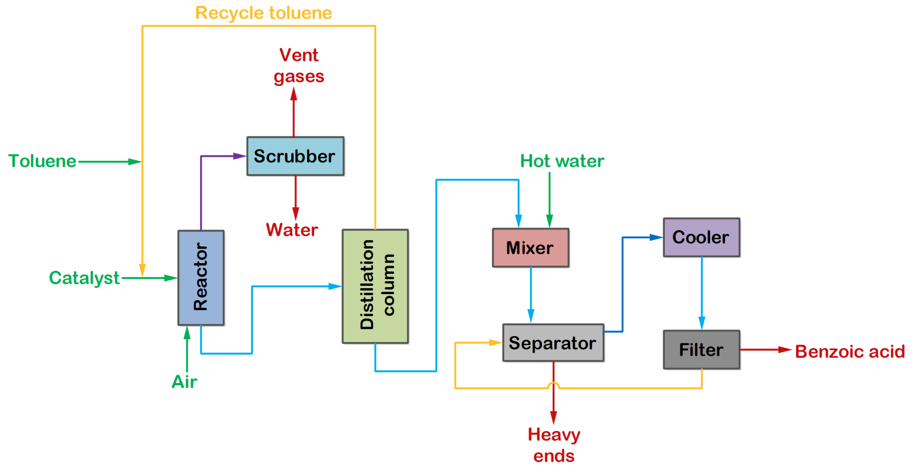
Figure: Manufacture of Benzoic acid from Toluene by air oxidation
